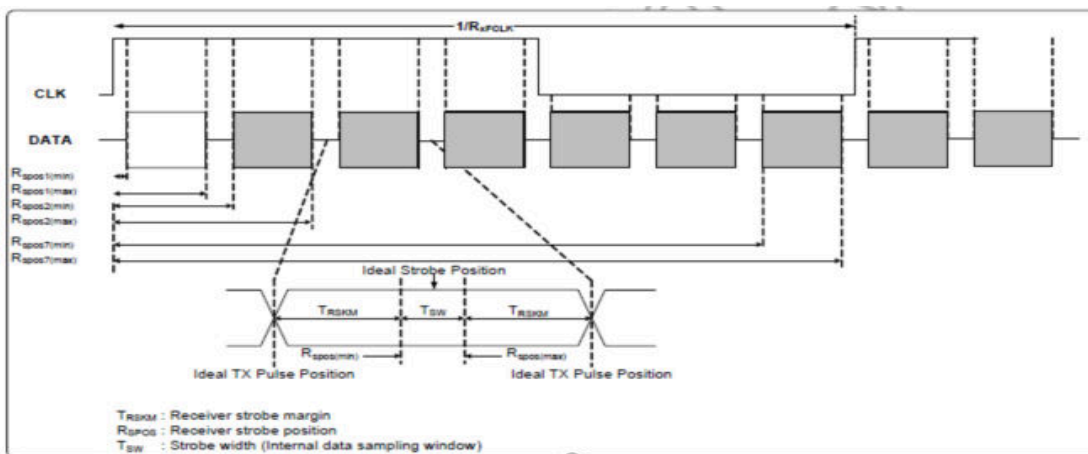
LVDS figure
